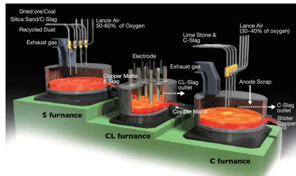
The Mitsubishi Process achieves industry-leading environmental load reduction.
